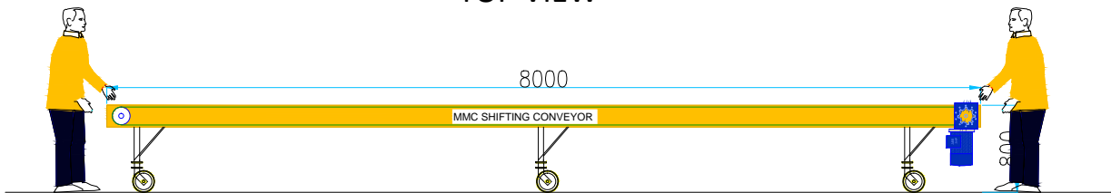
SIDE VIEW
