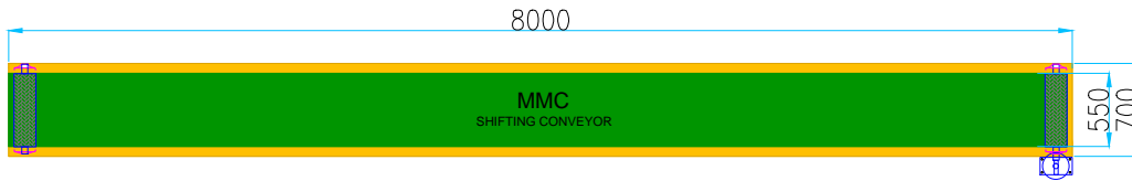
TOP VIEW
